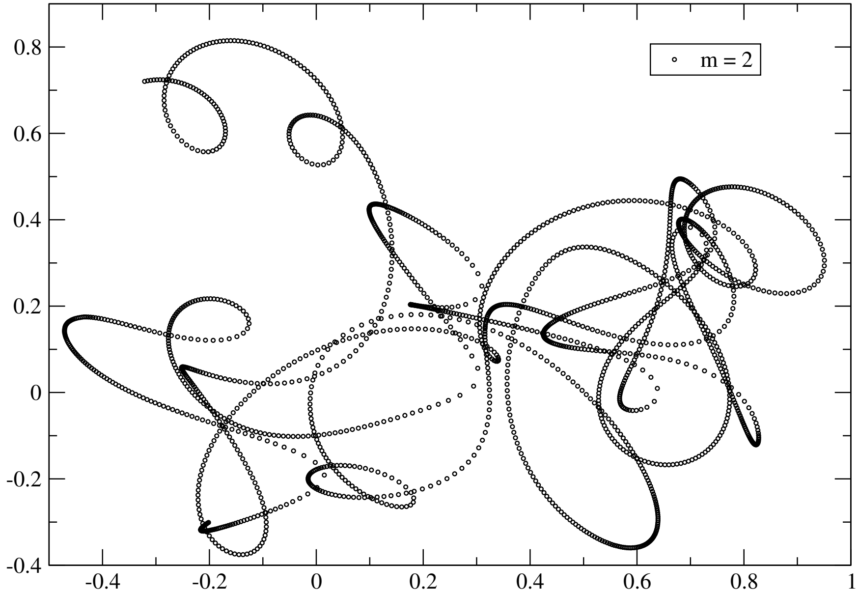
9 bodies in three dimensions: "central" body only
