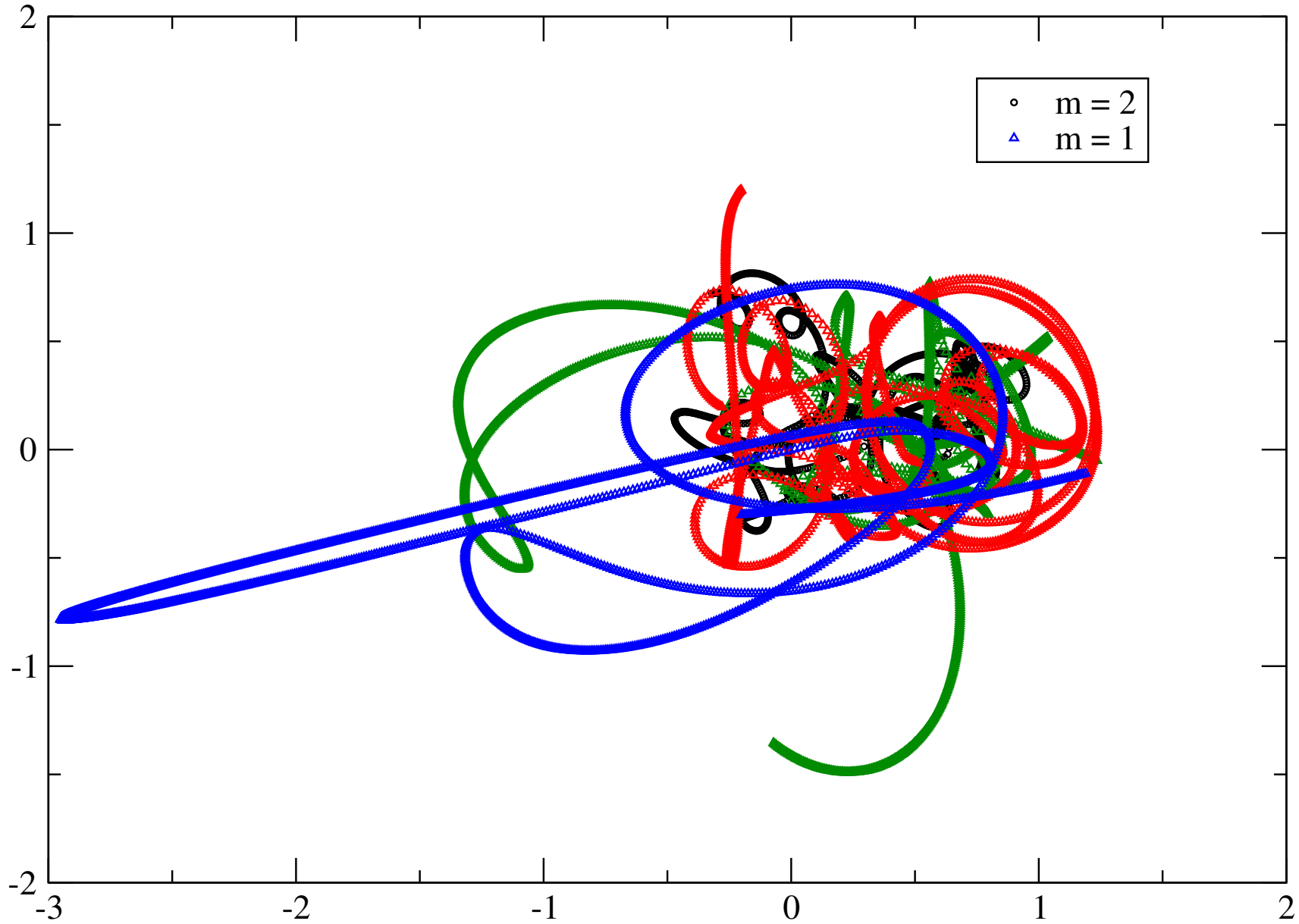
9 bodies in three dimensions: four light bodies escape
